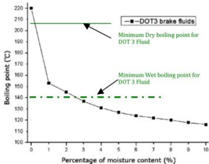
FIG. 6—Lowering of boiling point of DOT3 brake fluids with increasing moisture content.
