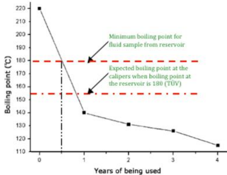
FIG. 7—Lowering of boiling point after use of DOT3 brake fluids (75 % RH).
